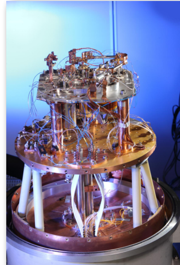
EASYCOOL – A 50MK CONTINUOUS REFRIGERATOR
